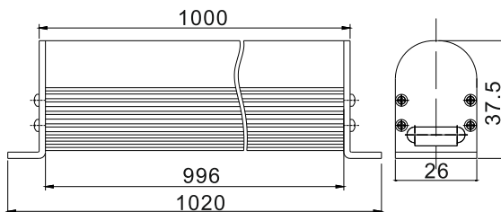
2 mounting holes \varnothing=4.0\text{mm}
