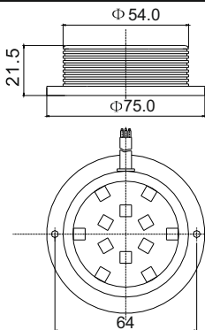
2 mounting holes \text{Ø}=5.0\text{mm} , distance: 64mm
